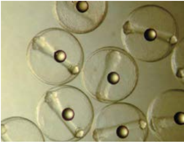
Fig. 2. Fertilized summer flounder eggs.
