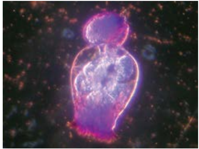
Fig. 4. Stained rotifer with egg
