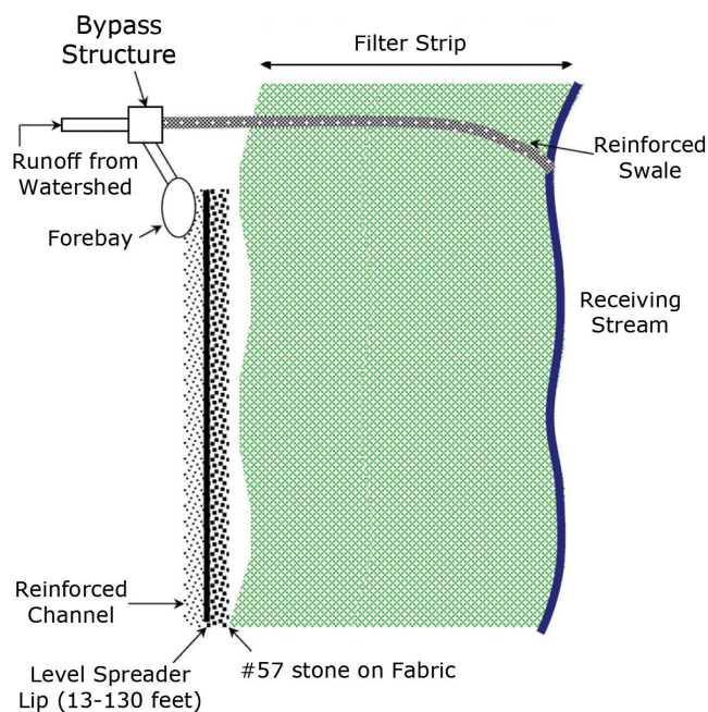
Figure 2. Plan view of sheet flow to open space Virginia Department of Environmental Quality (VA-DEQ 2011).
